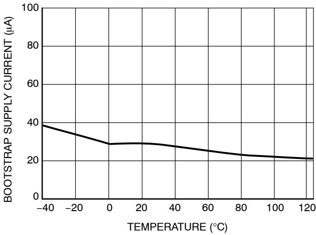
Figure 24. High Side Supply Current vs. Temperature
